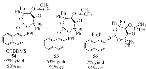
Scheme 11. Taddol-based phosphane-phosphite ligands
